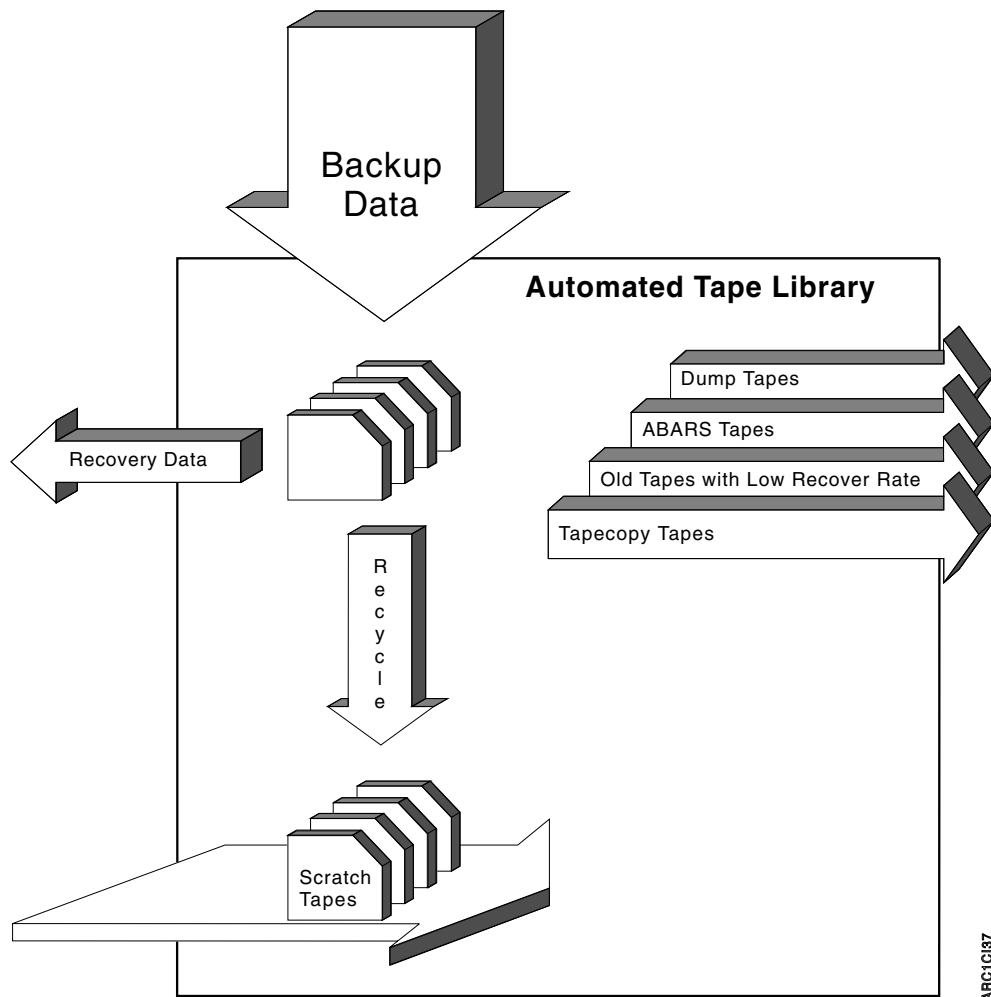
Figure 70. Overview of Implementing Backup in an Automated Tape Library
