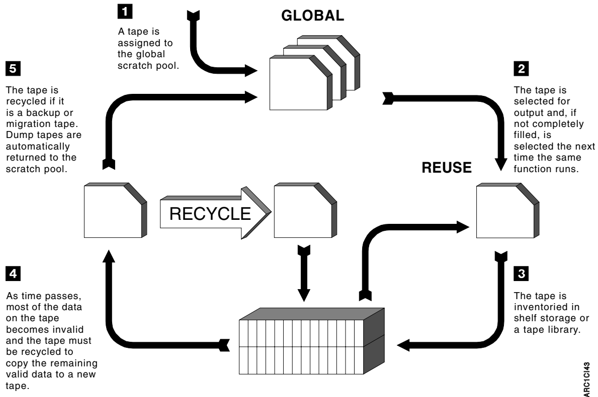
Figure 75. Recommended Tape Processing Environment that Maximizes Tape Capacity. This tape environment differs from the performance tape environment only in the way partially filled tapes are managed. Because partially filled tapes are selected the next time the same function runs, the tape's media is fully utilized.
