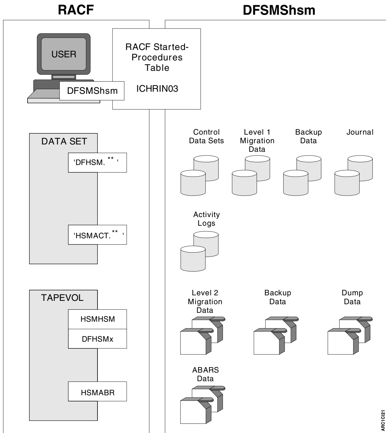
Figure 66. Overview of DFSMSHsm with RACF Environment
