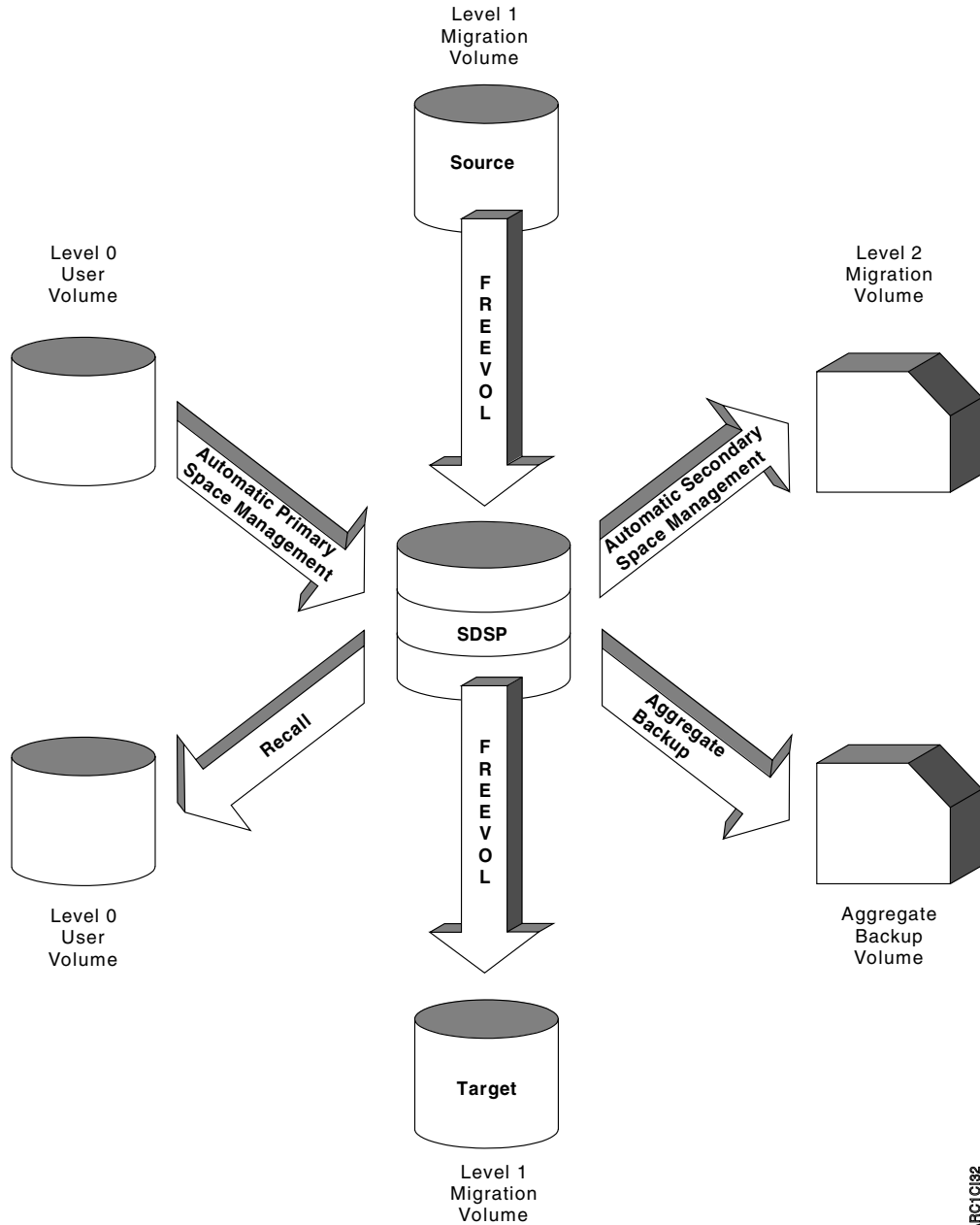
Figure 17. The SDSP Data Set Contention Environment
