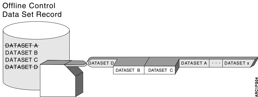
Figure 79. Tape Data Set Copy Invalidation. As migrated data sets are recalled and as backup versions expire, the data set entries in the OCDS become invalid. Invalid data sets remain on the tape, however, until the tape is recycled.
