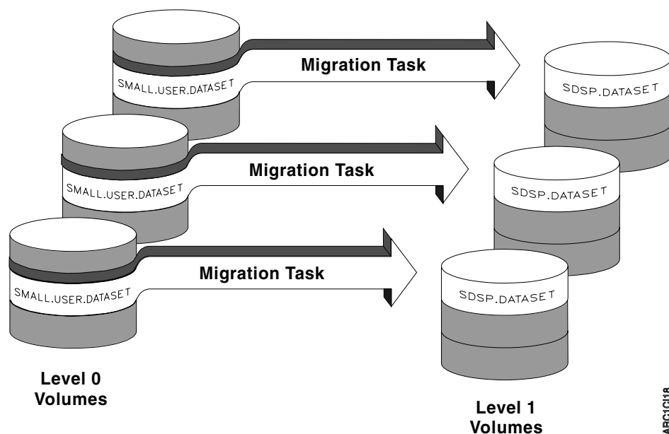
Figure 18. Part 1—Ideal Multitasking Migration. Three migration tasks migrate three small user data sets to three level-1 migration volumes on which SDSP data sets are defined.
