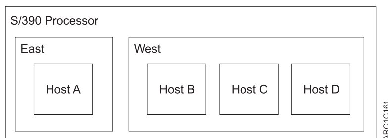
Figure 82. Example Configuration for a Multiple DFSMSHsm-Host Environment
