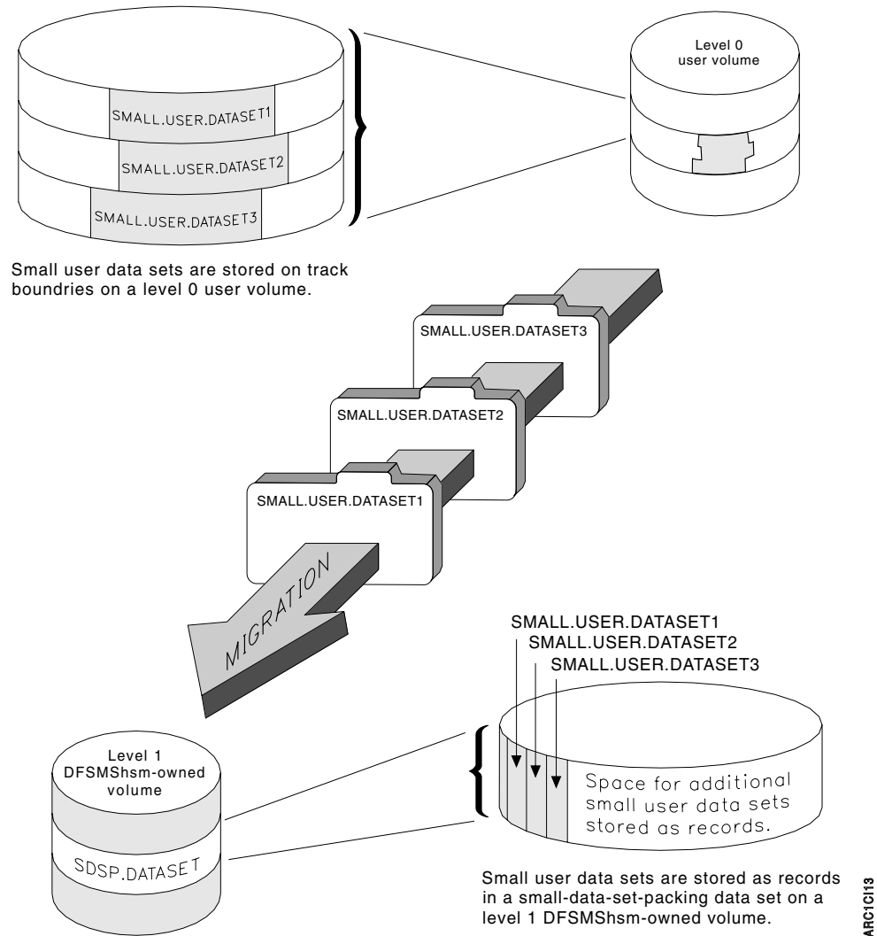
Figure 16. Small-Data-Set-Packing Data Set Overview
