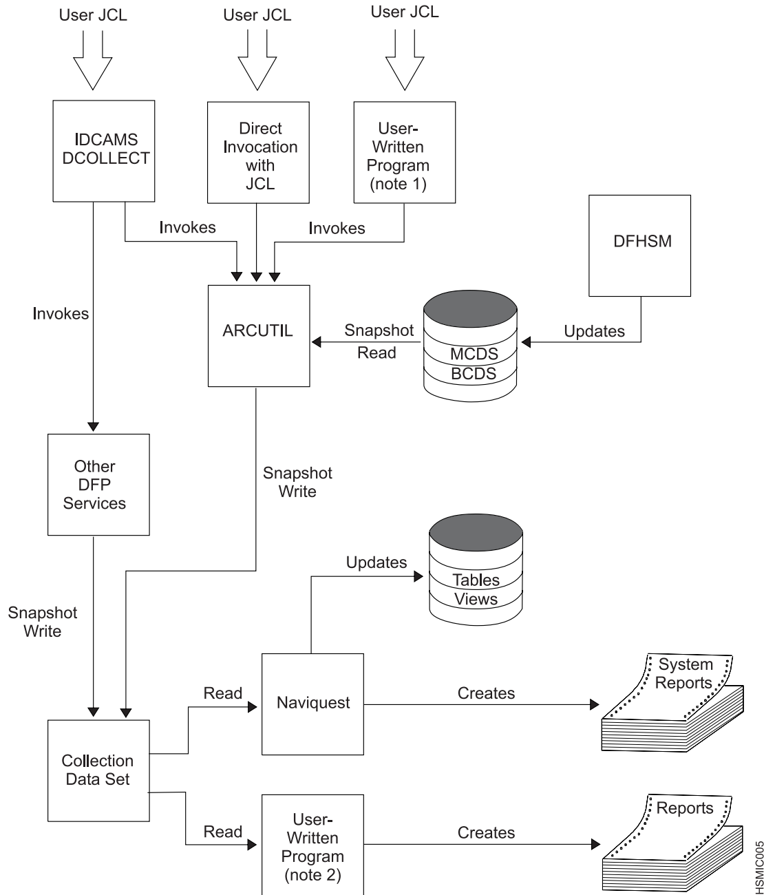
Figure 98. Data Collection Overview
