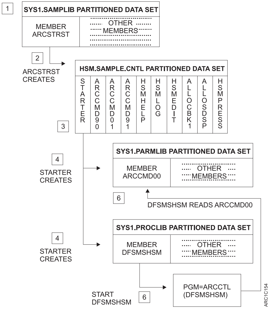
Figure 33. Starter Set Overview
