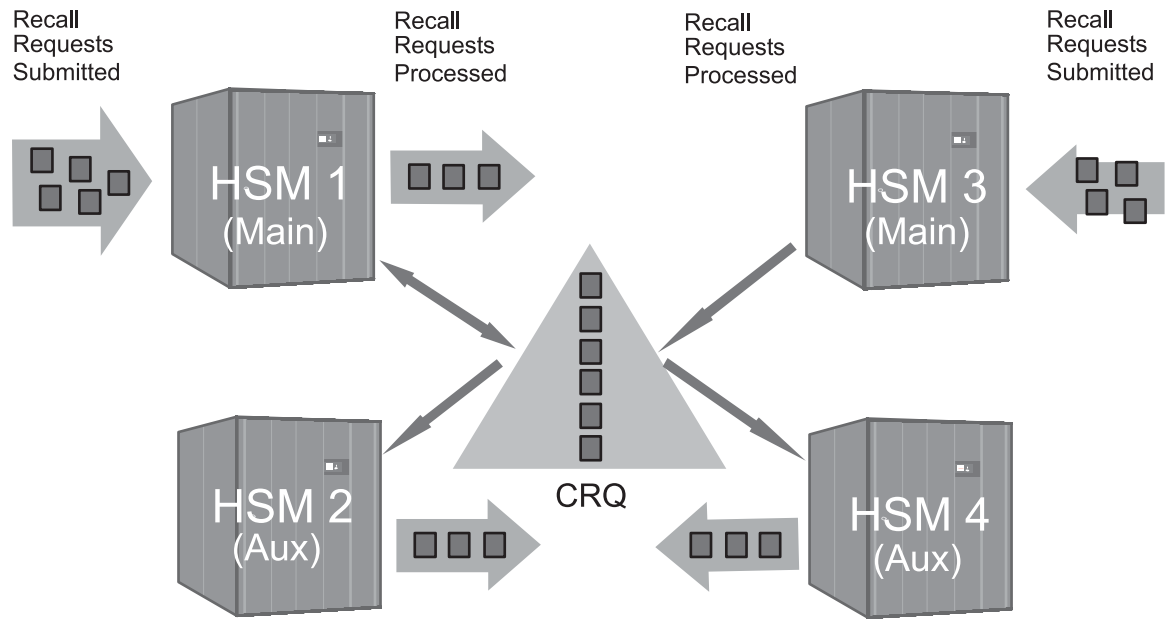
Figure 88. Overview of CRQplex Recall Servers
