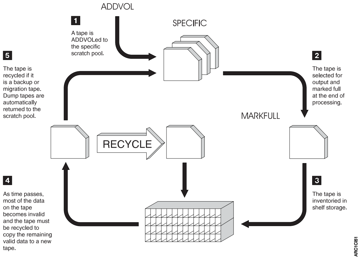
Figure 77. Environment For Specific Scratch Mounts. In this environment, DFSMShsm manages tapes and requests specific tapes to be mounted. An operator is required for all tape mounts; however, separate ranges of tapes can be assigned to DFSMShsm and to other users and managed according to the requirements of each user. Note that DFSMShsm treats a partial migration tape that is taken away for recall as if you had specified SETSYS PARTIALTAPE(REUSE).
