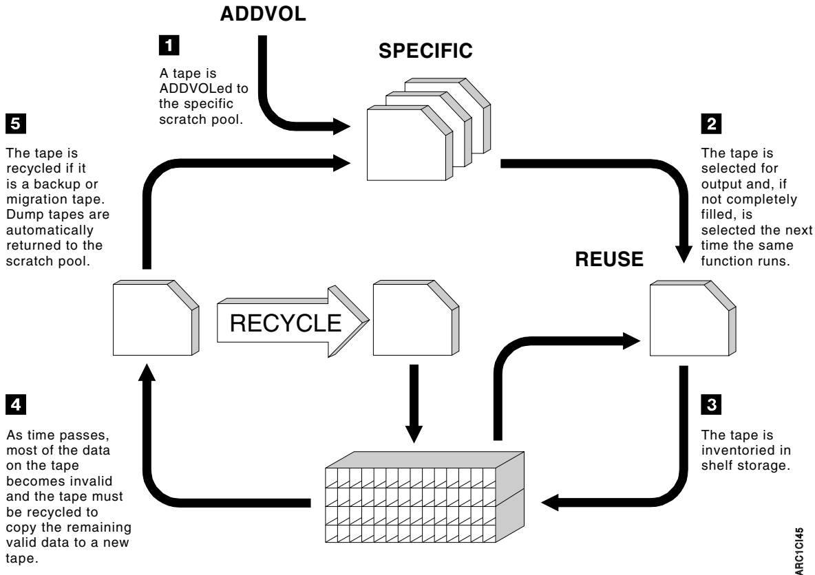
Figure 76. Recommended Environment For Managing Separate Ranges of Tapes. In this environment, operations requests a list of empty tapes. The initial mount request for migration, backup, or their recycle is for a specific tape. After the initial tape is mounted, operations either preloads the empty tapes into cartridge loaders or responds to mount requests.
