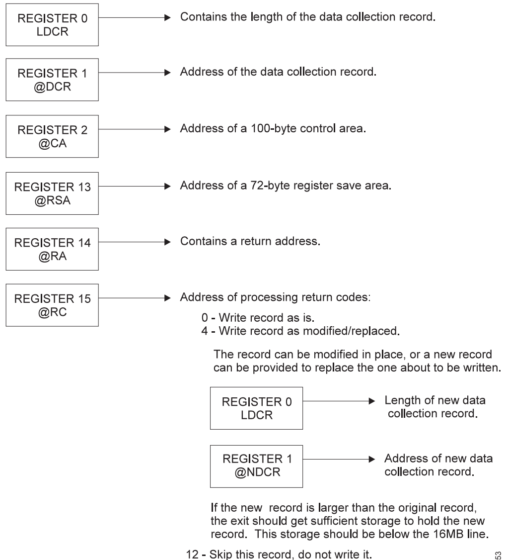
Figure 104. Exit for Data-Collection Support
