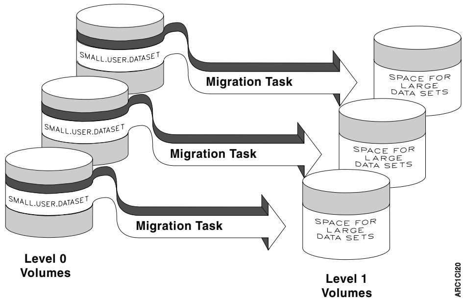
Figure 20. Part 3—All SDSP Data Sets Are Full. The small user data sets migrate as large data sets to the level-1 migration volumes.
