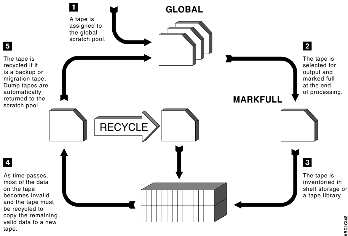
Figure 74. Recommended Performance Tape Processing Environment. This is the most versatile and easily managed of the recommended tape environments. This environment is recommended for both library and nonlibrary tape environments. Note that DFSMSHsm treats a partial migration tape that is taken away for recall as if you had specified SETSYS PARTIALTAPE(REUSE).
