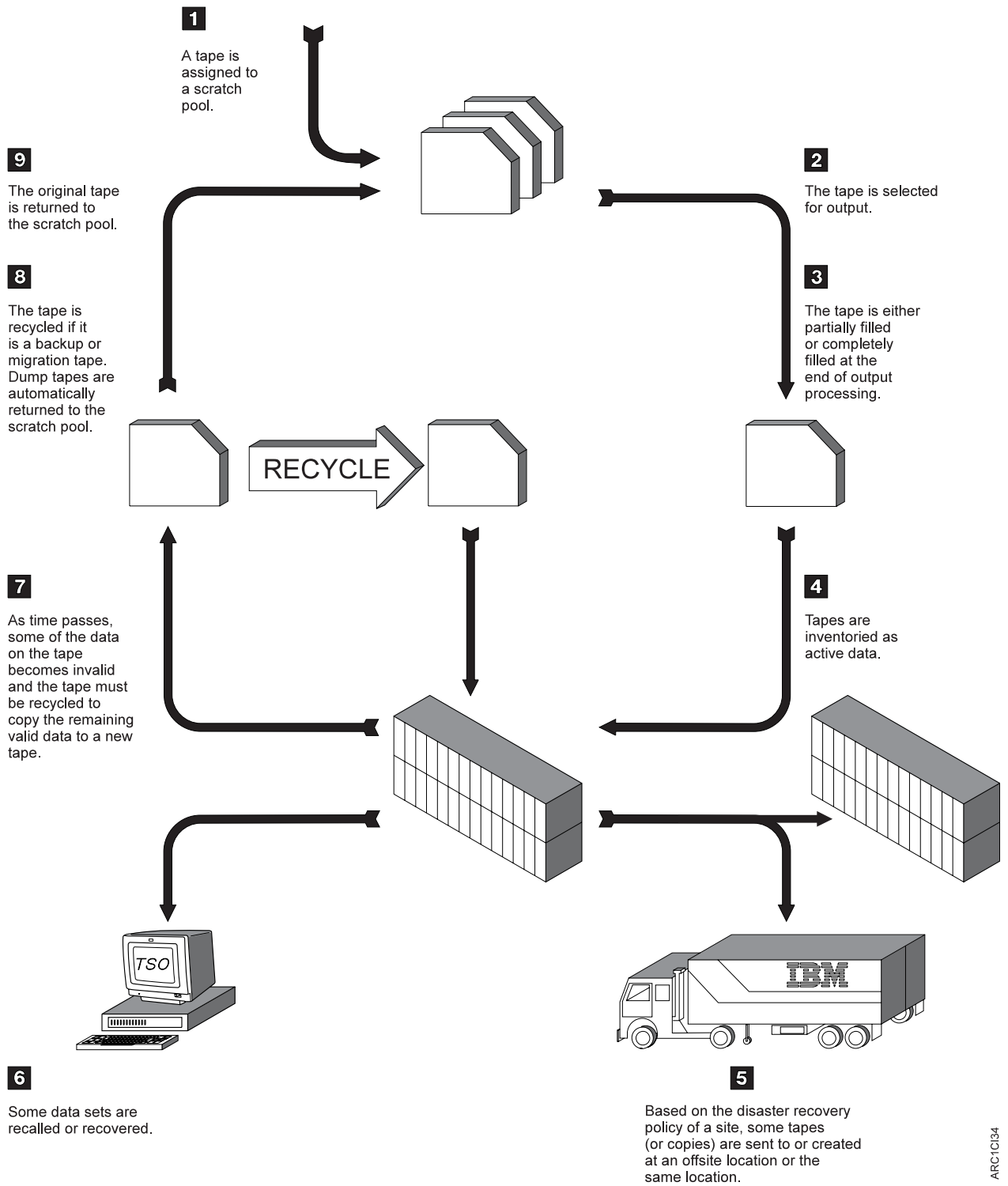
Figure 72. Life Cycle of a Tape. The life cycle of a tape is determined by the SETSYS commands you specify that manage the tape as it enters a scratch pool, is selected for output, is inventoried as active data, is recycled (if it is a backup or migration tape), and finally is returned to the scratch pool.
