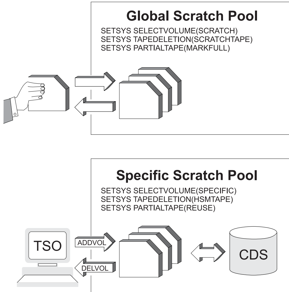
Figure 73. Overview of Tape Scratch Pools. A global scratch pool does not require making tapes known to DFSMSHsm because they are managed by a tape management product (DFSMSrmm, for example). Global scratch pools are recommended for SMS-managed tape libraries and unattended operation.
