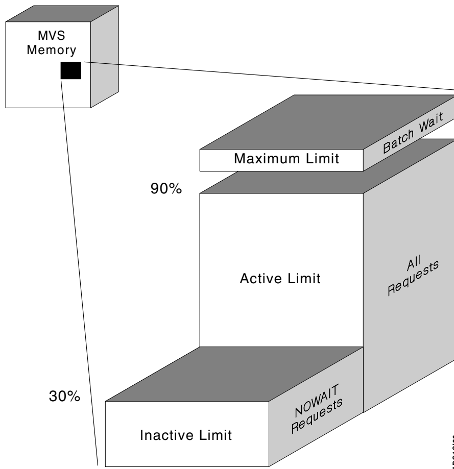
Figure 27. Overview of Common Service Area Storage
