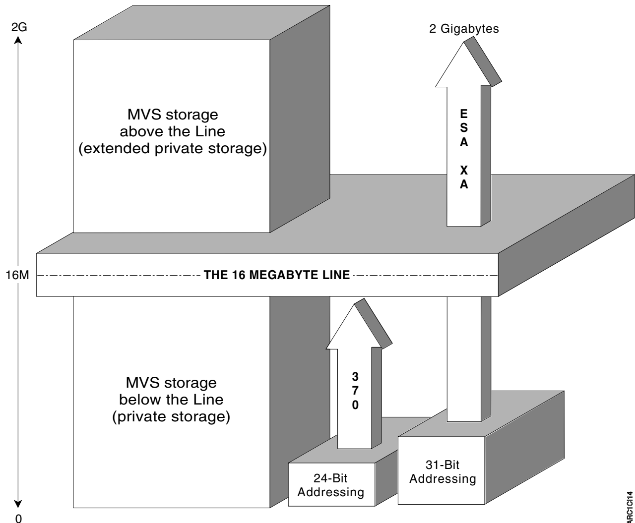
Figure 89. The MVS Storage Environment
